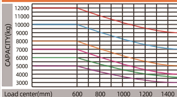
Load curve
